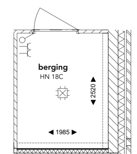
00 begane grond - 1:50
